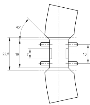
2GX13 cap, IEC 60061
